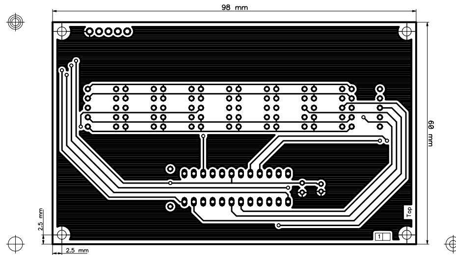
Expansion Board - 8x7-Segments - (09/2017) SCALE: 100%
