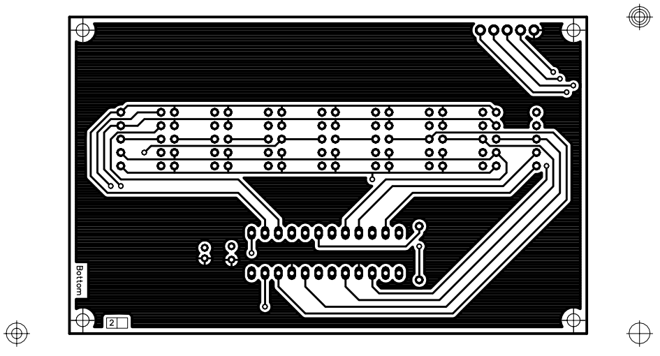
Expansion Board - 8x7-segments - (09\2017) SCALE: 100%
