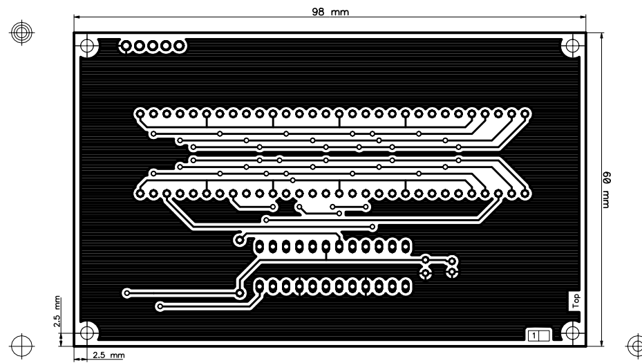
Expansion Board - 6x7-Segments - (09/2017) SCALE: 100%
