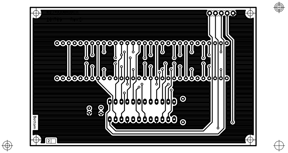
Expansion Board - 6x7-segments - (09\2017) SCALE: 100%
